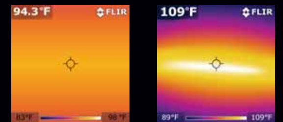
Lower Temperature with Thermal Break (Northwest Door)
